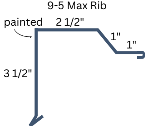
Rake & Gable
