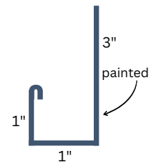
J Channel
