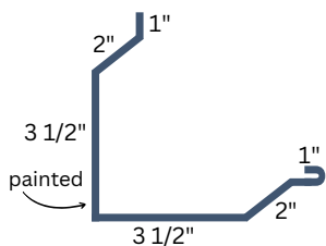
Corner & Gable
