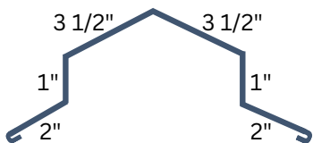
Ridge Cap
