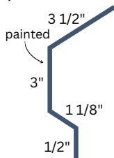
Drip Cover w/ Purlins
