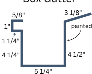
Box Gutter
