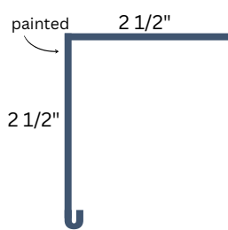
Eave Trim
