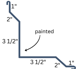
Inside Corner
