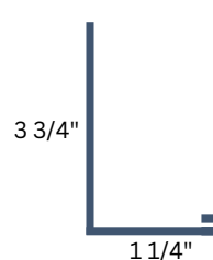
Base
